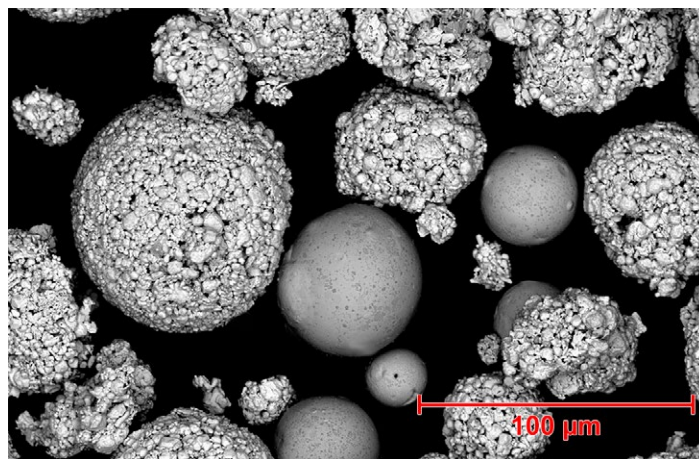
SEM Photomicrograph of Amdry 1371 showing the morphology of this blended powder product
