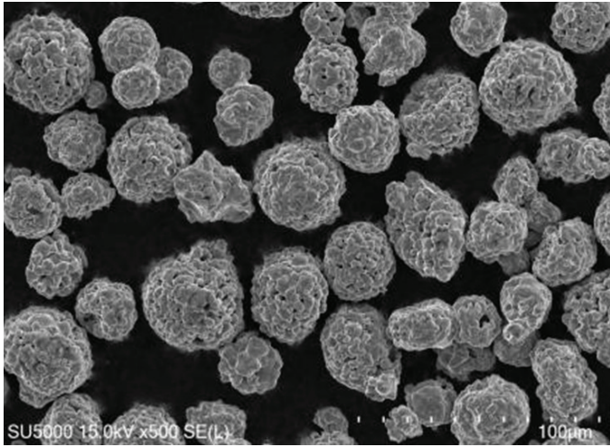
Metallography of WallCarb™ 75/25 HVOF powder showing spherical particles 500X
